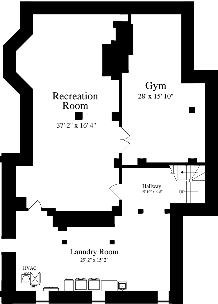
LOWER LEVEL (ceiling = 7' 9")
