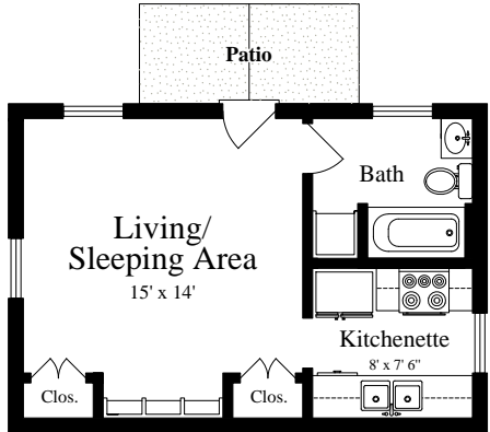
FIRST FLOOR - Guest House (vaulted ceiling = 14' 8")
